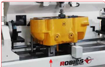
LARGE IN-LINE HEADS USING TWO DEGREE TILT FIXTURE
