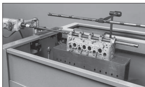
Cylinder head being honed on CH-100 Honing Machine with a hand fed Porta-Hone.
